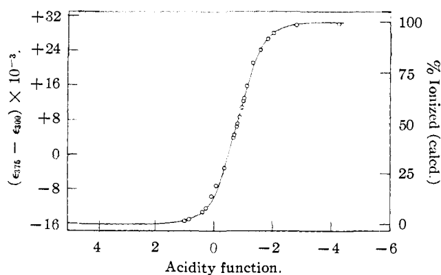
Fig. 6.—4'-Methoxyflavone: acidity function vs. (\epsilon_{375} - \epsilon_{300}) ; points from spectral data, curve calculated for pK_a = 0.8 .
