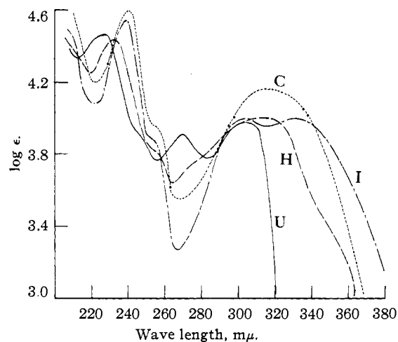
Fig. 5.—Absorption spectra of 2',3,4',6'-tetramethylflavone: U, —, in 95% ethanol; H, — — — —, in 42% H 2 SO 4 ; I, — · — · —, in 68.6% H 2 SO 4 ; C, · · · · ·, in 95.5% H 2 SO 4 .
