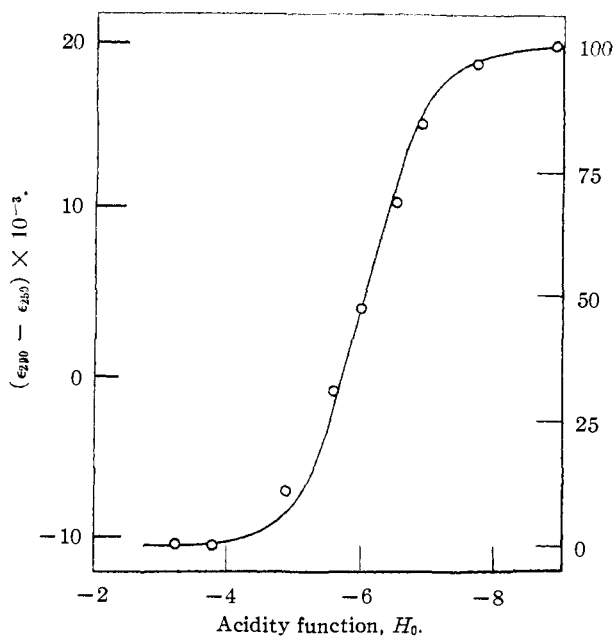
Fig. 7.—Acetophenone: acidity function vs. (\epsilon_{290} - \epsilon_{280}) ; points from spectral data (ref. 11); curve calculated for pK_a = 6.05 .
