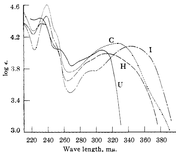
Fig. 4.—Absorption spectra of 2',4',6'-trimethylflavone: U, —, in 95% ethanol; H, — — — —, in 36.2% H 2 SO 4 ; I, — · — · —, in 66.5% H 2 SO 4 ; C, · · · · ·, in 93.1% H 2 SO 4 .
